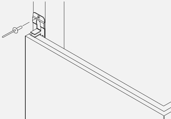
E - Support plate vertical 2 flaps
