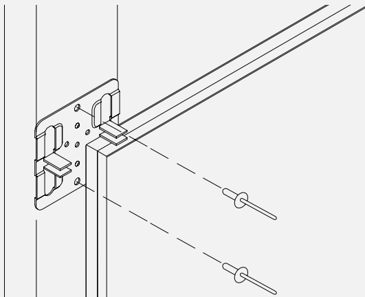
C - Support plate horizontal 4 flaps
