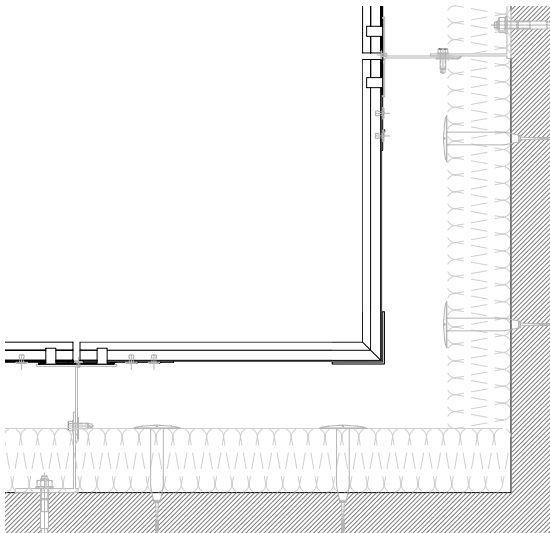
▼ Internal Corner
