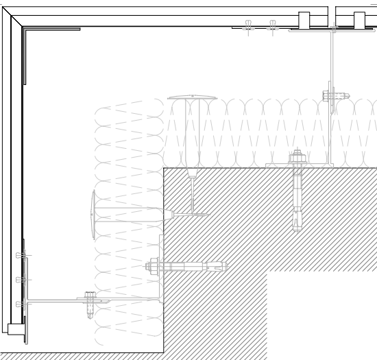
▼ External Corner
