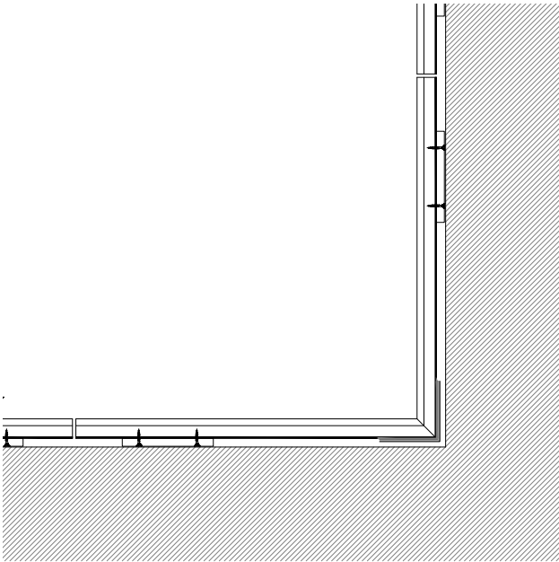
▼ Internal Corner
