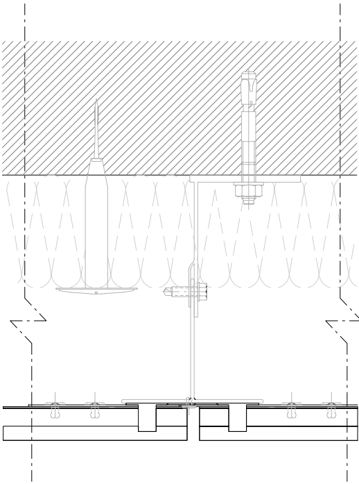
▼ Horizontal Section
