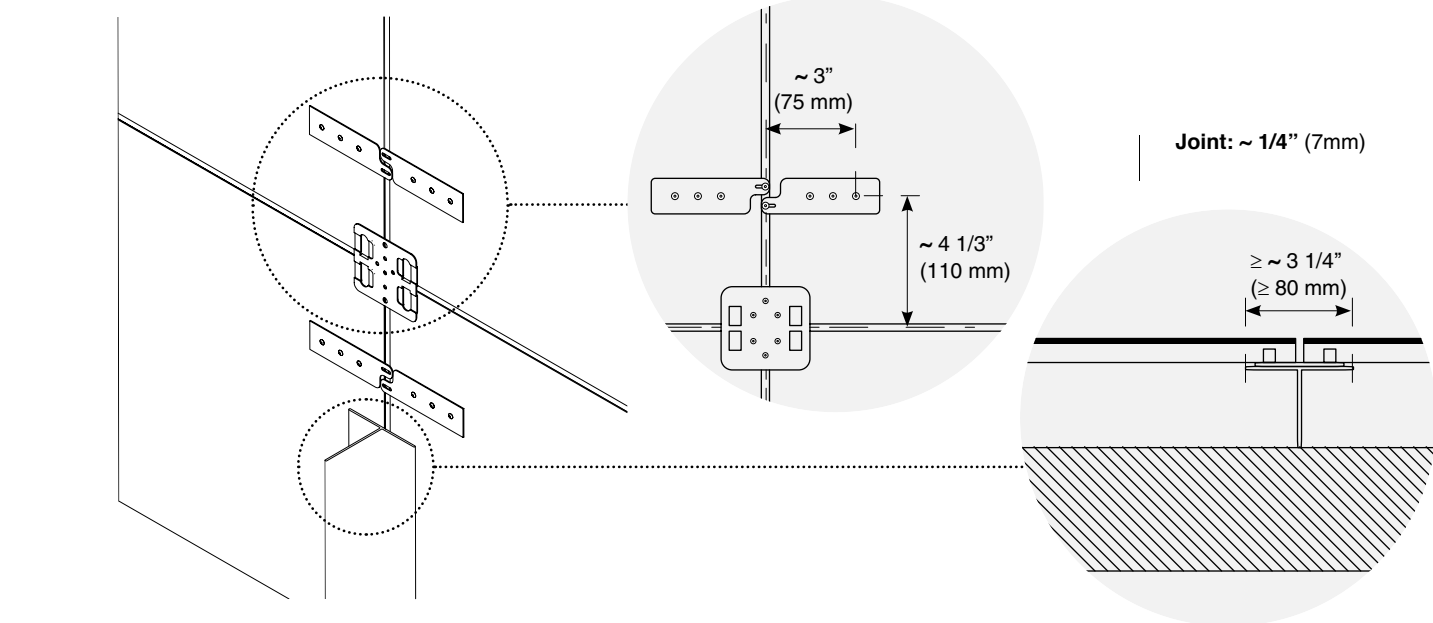
▼ Back view
