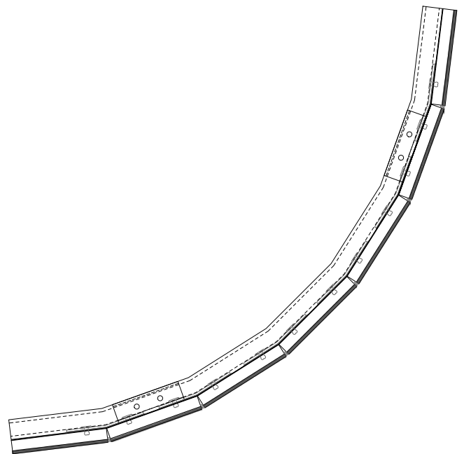
Segmented curved panel
